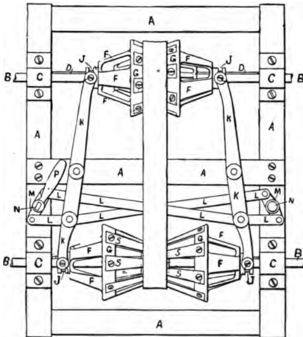
FIG. 248.—Diagram of a Variable Cone Pulley Transmission.
